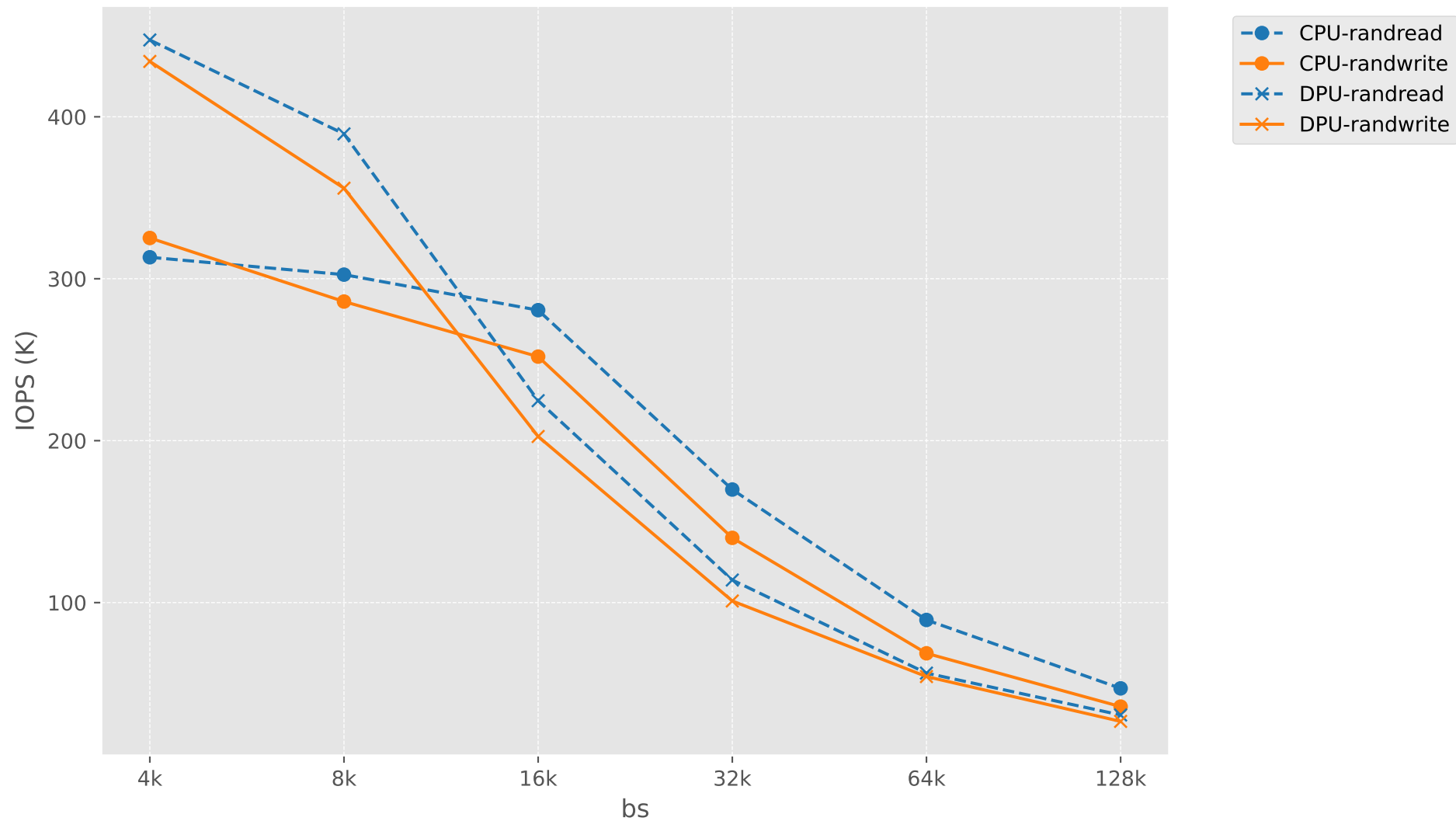
IOPS vs bs
